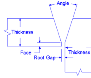
CORNER SINGLE VEE
