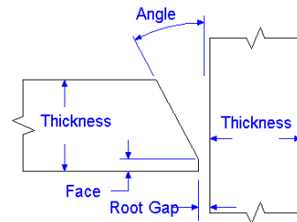
'T' JOINT SINGLE BEVEL
