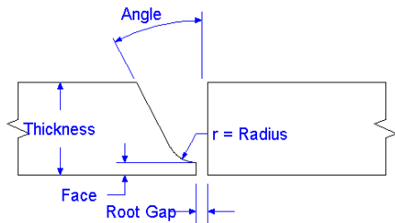
SINGLE 'J'
