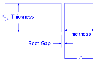
CORNER SQUARE
