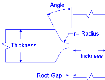
'T' JOINT DOUBLE 'J'
