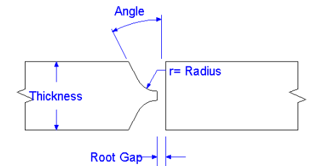
DOUBLE 'J'
