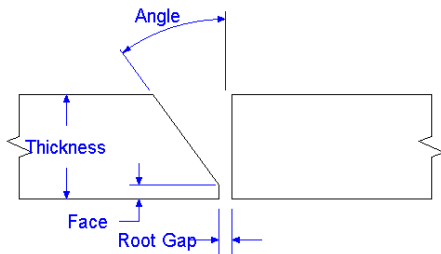
SINGLE BEVEL
