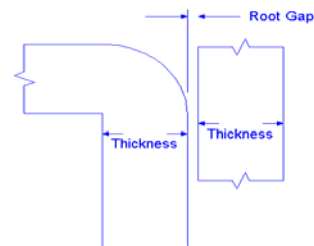
'T' JOINT (FLARE) SINGLE BEVEL
