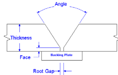
SINGLE VEE with BACKING
