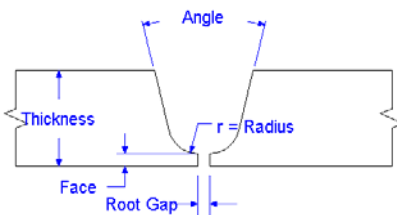
SINGLE 'U'
