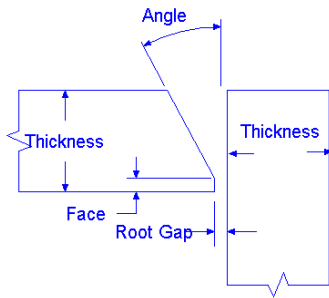
CORNER SINGLE BEVEL
