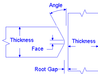
'T' JOINT DOUBLE BEVEL
