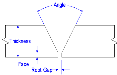
SINGLE VEE
