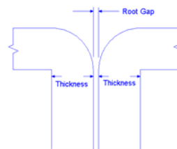
'T' JOINT (FLARE) SINGLE VEE
