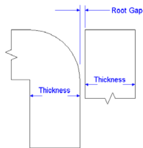
CORNER (FLARE) SINGLE BEVEL
