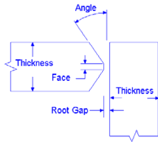
CORNER DOUBLE BEVEL
